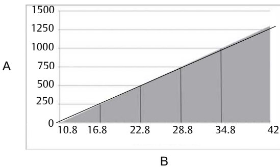
Figure 5-1: Load limitation
