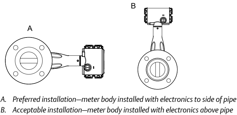
Figure 2-2: Horizontal installation
