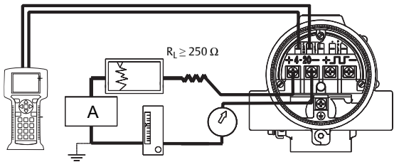
Figure 5-3: 4–20 mA wiring
