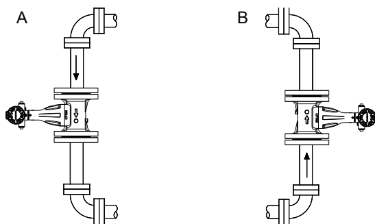
Figure 2-1: Vertical installation
