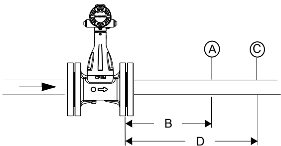
Figure 2-5: Upstream/Downstream piping
