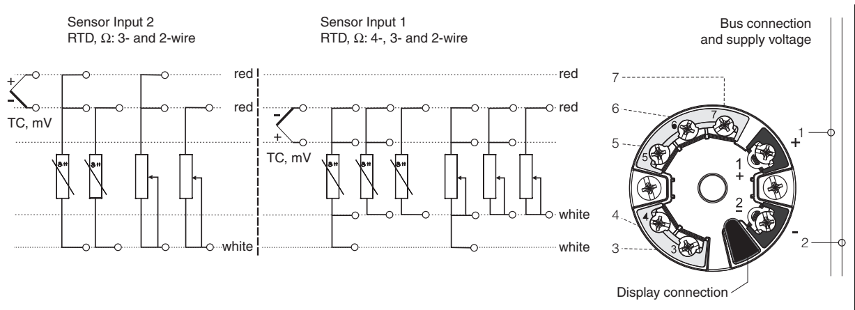
Figure 2. Input Connections – Basic Transmitter and Universal Housing
