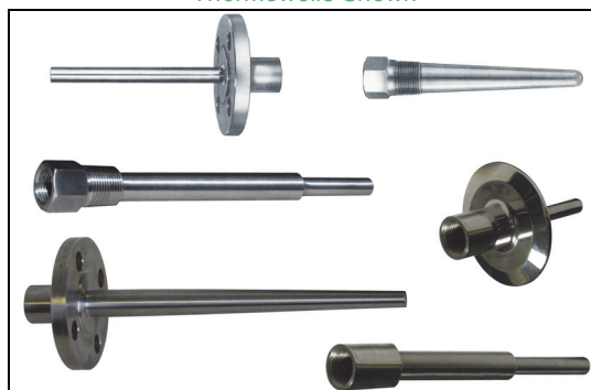
Figure 6. Typical W-Series and T-Series Thermowells Shown
