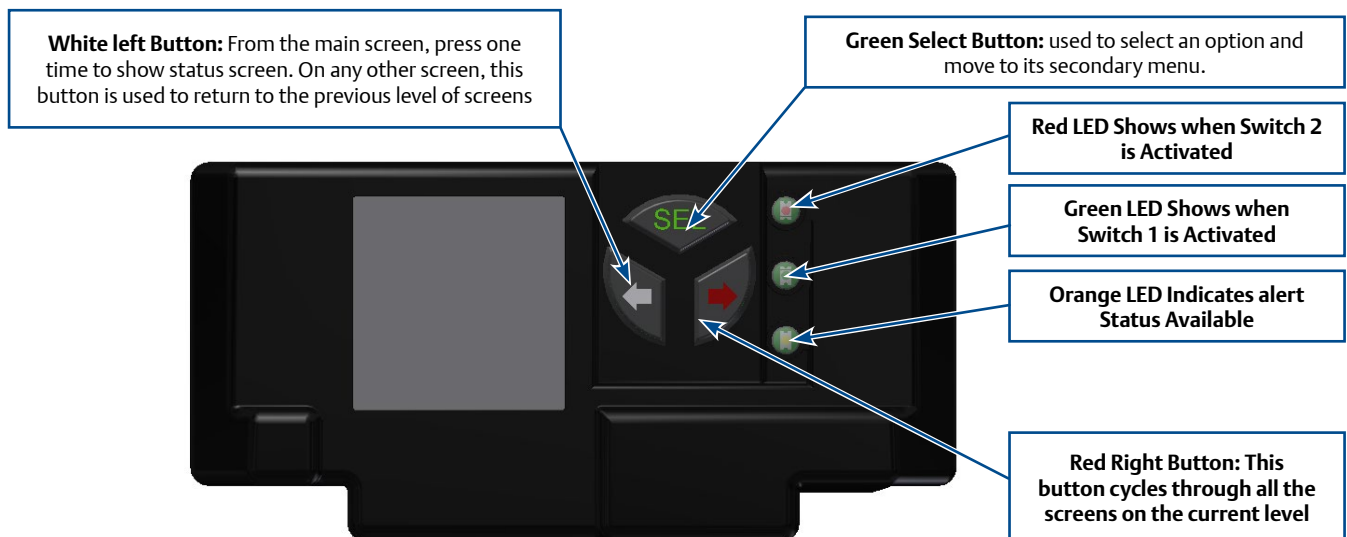
Figure 3: Buttons and Indicator Lights
