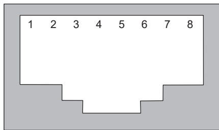
Figure Front View of RJ45 Jack
