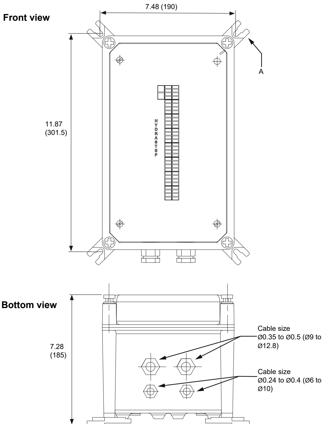
Figure 5. Hydrastep Wall Mount iP65 Remote Display (24683D)
