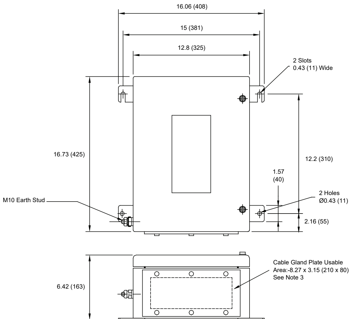
Figure 2. Hydrastep Enclosure
