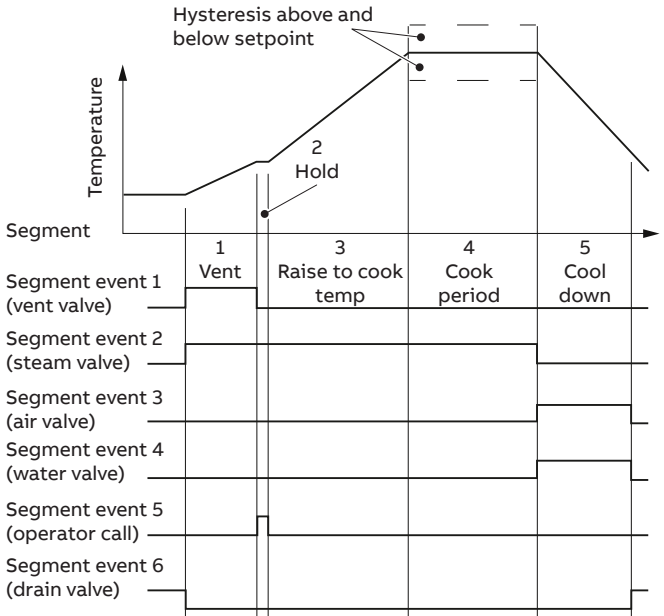
Figure 18 Profile control
