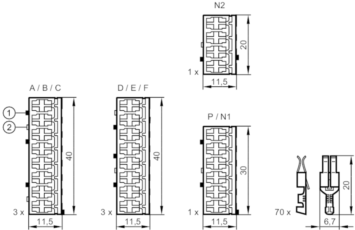
figure shows contact housing with closed covers view on contact plug-in side
