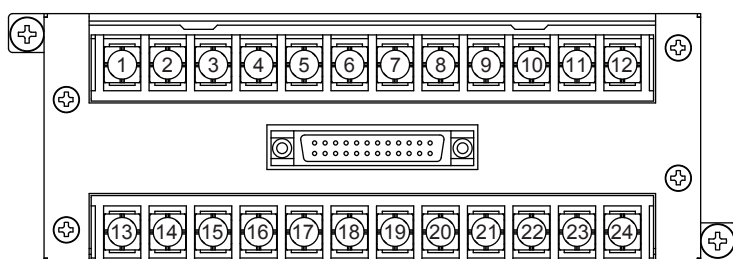
Expandable I/O Terminal Diagram
