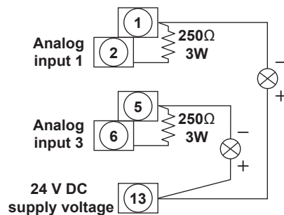
Connection of Transmitter Power Supply
