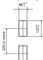
Panel Cutout Dimensions
