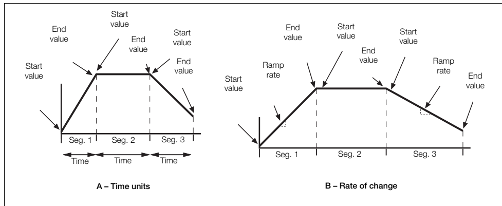
Fig. 7.1 Ramp Types
