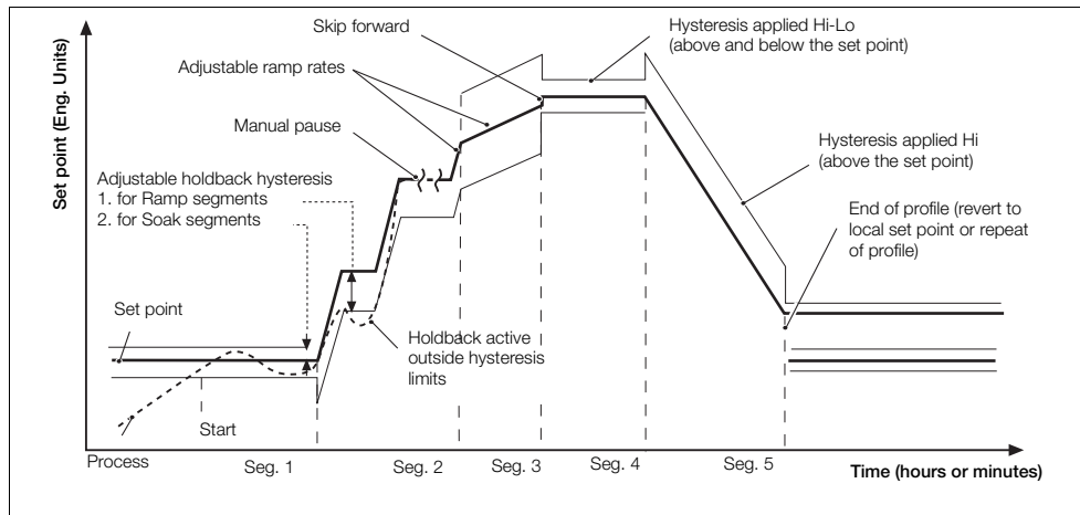
Fig. 7.2 Ramp Types
