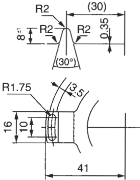
DETAIL OF SPRING PLATE
