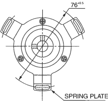
DETAIL OF SPRING PLATE
