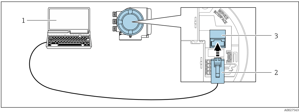
51 Connection via service interface (CDI-RJ45)
