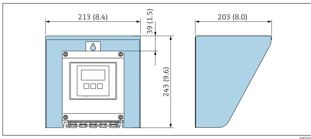
23 Weather protection cover for Proline 500 – digital
