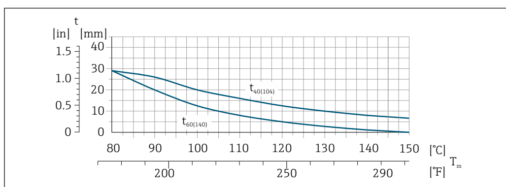
38 Maximum recommended insulation thickness depending on the temperature of the medium and the ambient temperature
