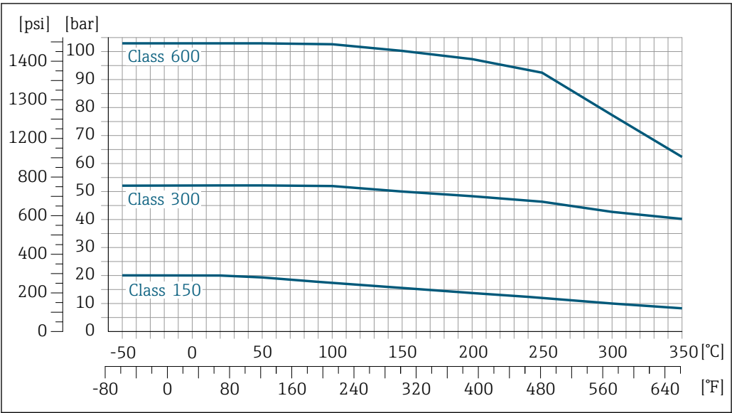
27 With flange material Alloy C22
