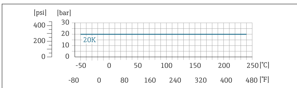
32 With flange material 1.4301 (F304); wetted parts Alloy C22
