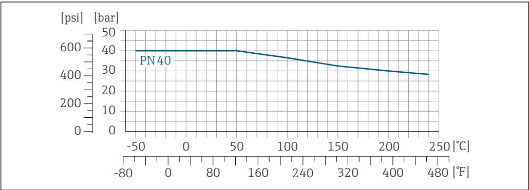
30 With flange material 1.4301 (F304); wetted parts Alloy C22
