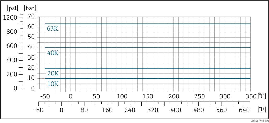
28 With flange material 1.4404 (F316/F316L), Alloy C22
