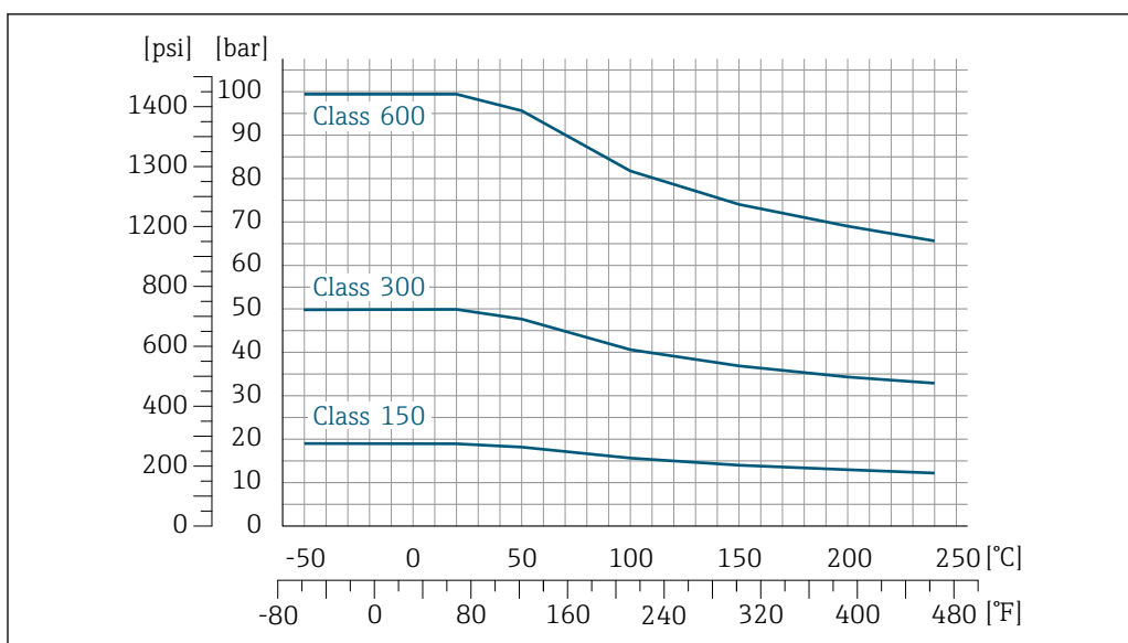
31 With flange material 1.4301 (F304); wetted parts Alloy C22
