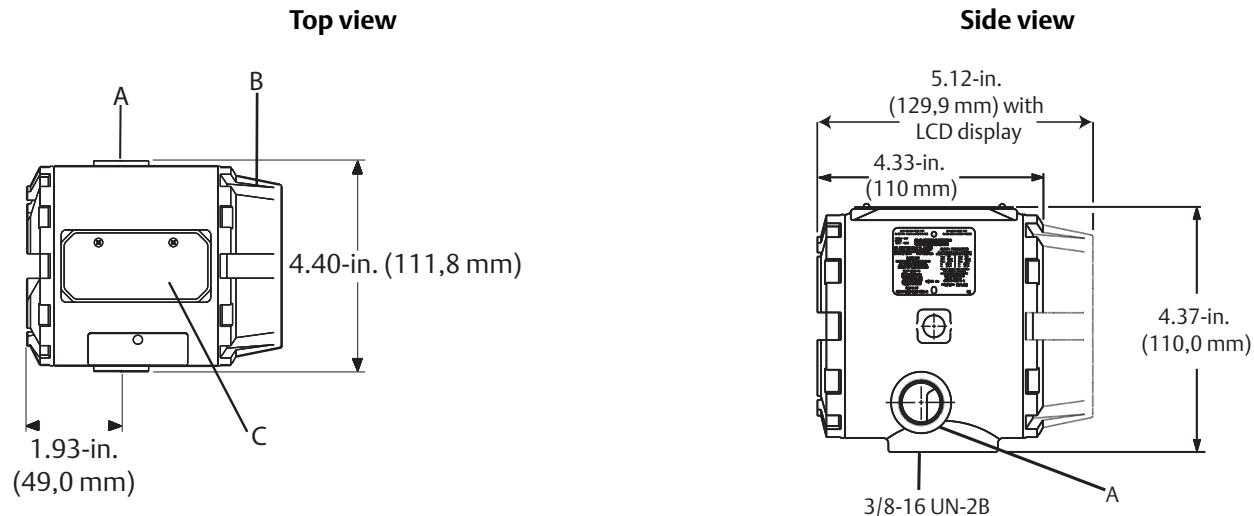
Figure 3. Transmitter
