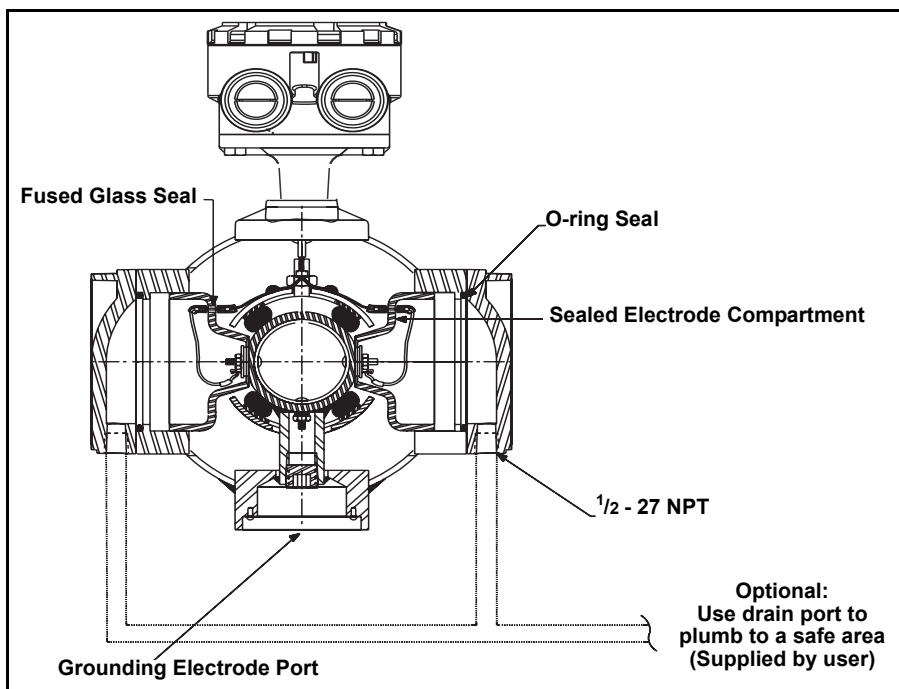
Figure 2-15. Housing Configuration — Sealed Electrode Compartment (Option Code W3)
