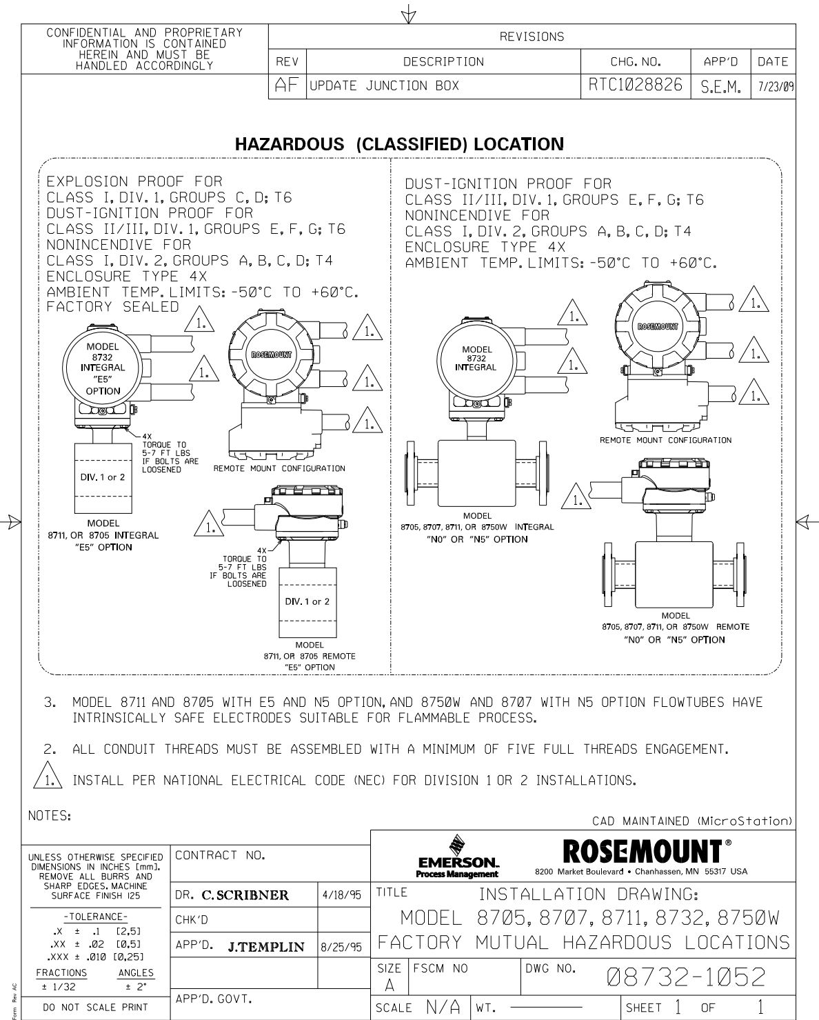
Figure B-16. Installation Drawings Factory Mutual Hazardous Location
