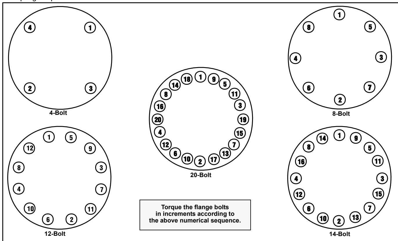
Figure 2-10. Flange Bolt Torquing Sequence
