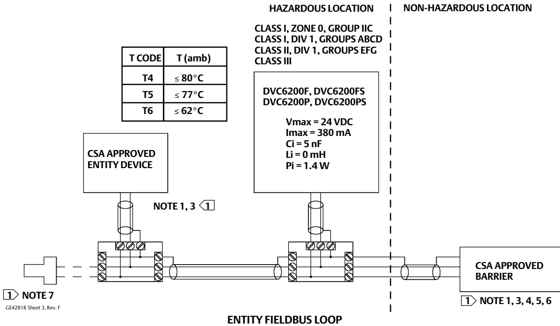
Figure 3. CSA Loop Schematics—FIELDVUE DVC6200f and DVC6200p
