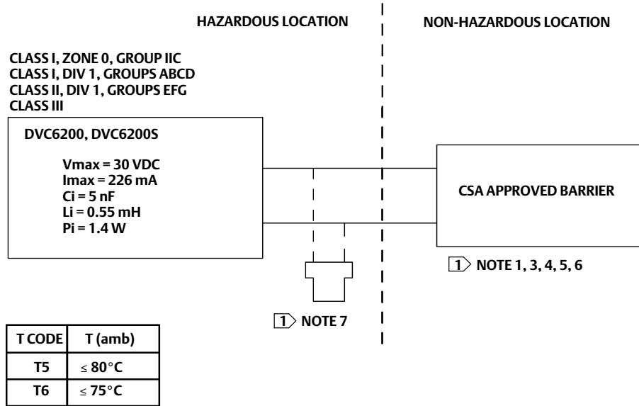
Figure 5. CSA Loop Schematic—FIELDVUE DVC6200 HW1
