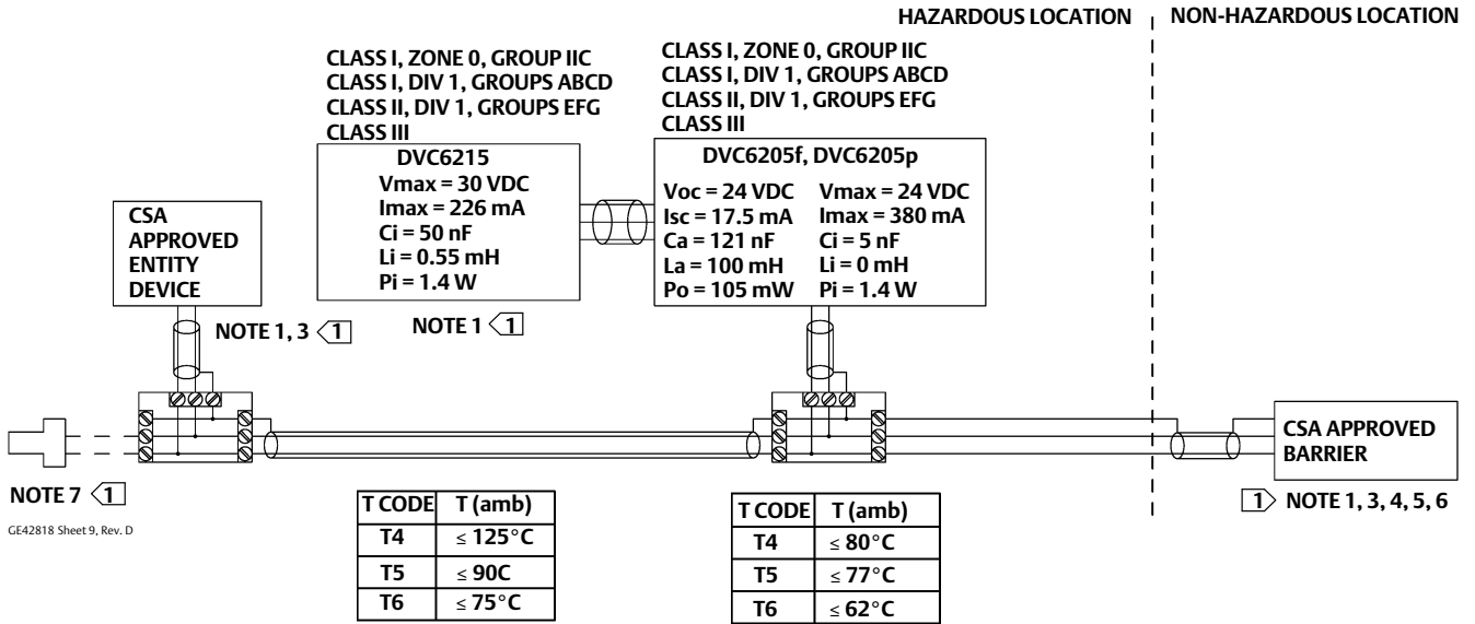
Figure 4. CSA Loop Schematics—FIELDVUE DVC6205f, DVC6205p, and DVC6215
