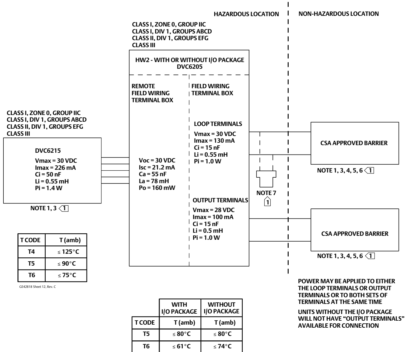
Figure 2. CSA Loop Schematics—FIELDVUE DVC6205, DVC6205 SIS, and DVC6215
