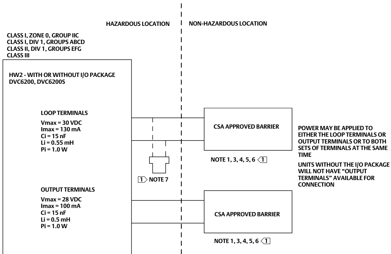
Figure 1. CSA Loop Schematics—FIELDVUE DVC6200 HW2 and DVC6200 SIS
