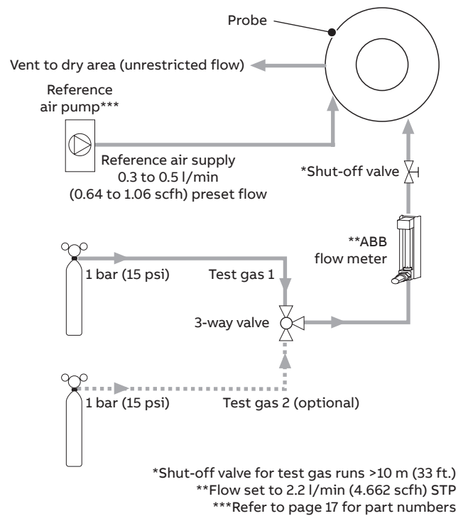
Non-AutoCal with test gas(es) and no restrictors
