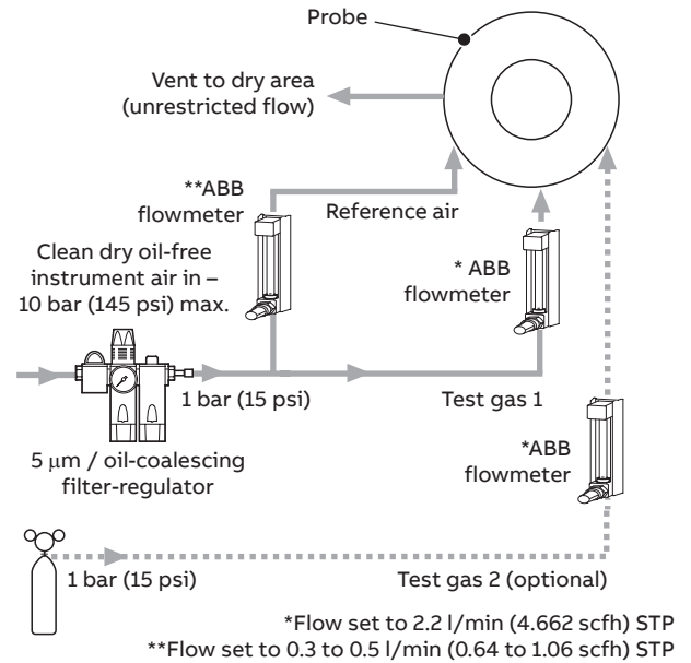
AutoCal with air supply and no restrictors
