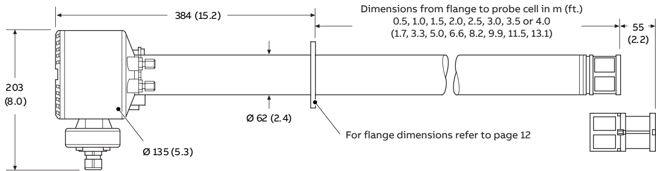
Overall dimensions – remote probe
