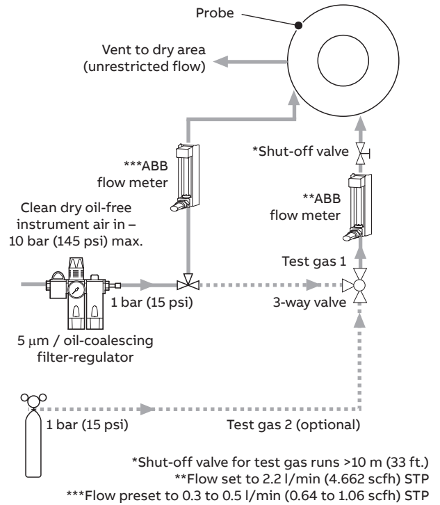
Non-AutoCal with air supply and no restrictors
