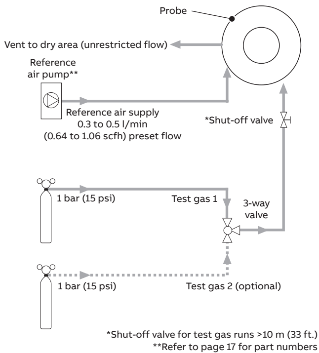
Non-AutoCal with test gas(es) and restrictors
