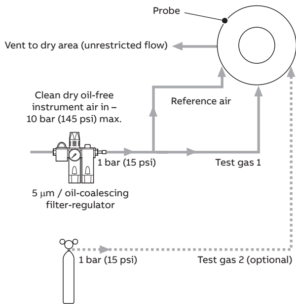
AutoCal with air supply and restrictors
