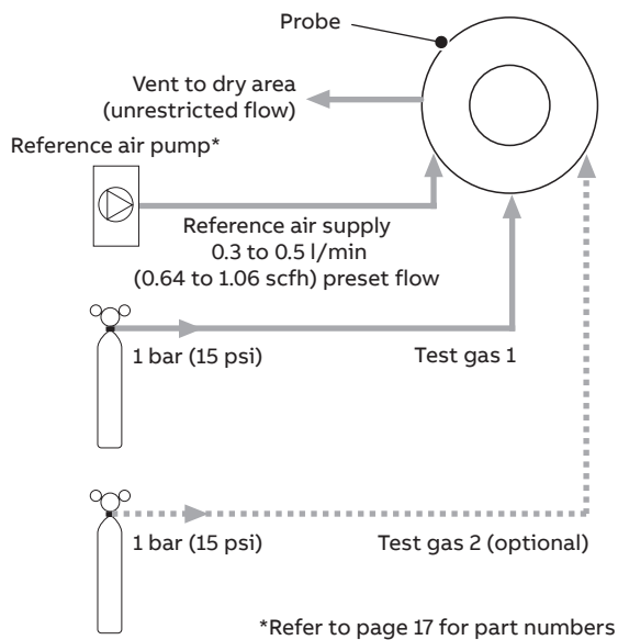
AutoCal with test gas(es) and restrictors
