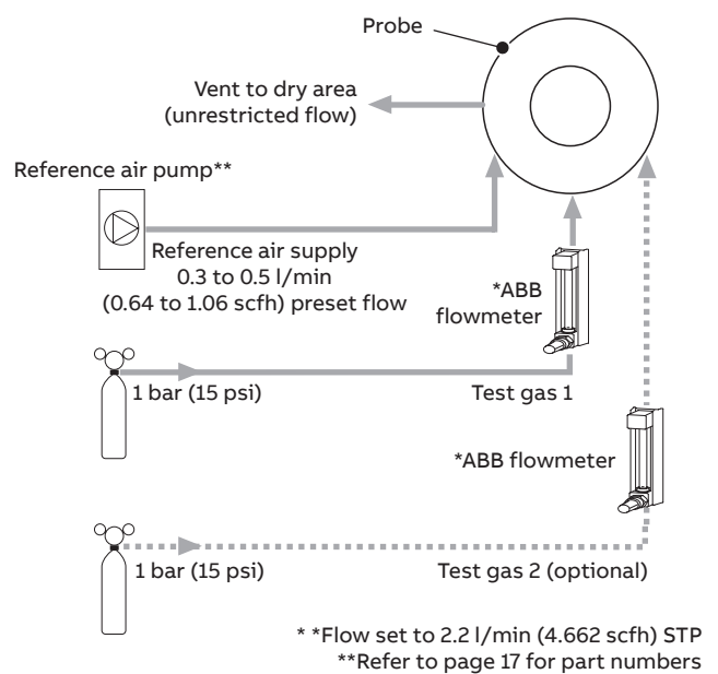
AutoCal with test gas(es) and no restrictors
