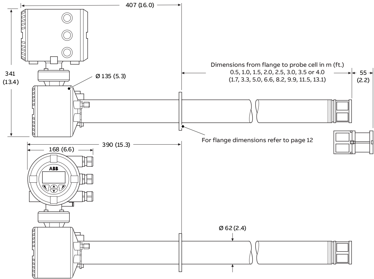
Overall dimensions – probe and integral transmitter
