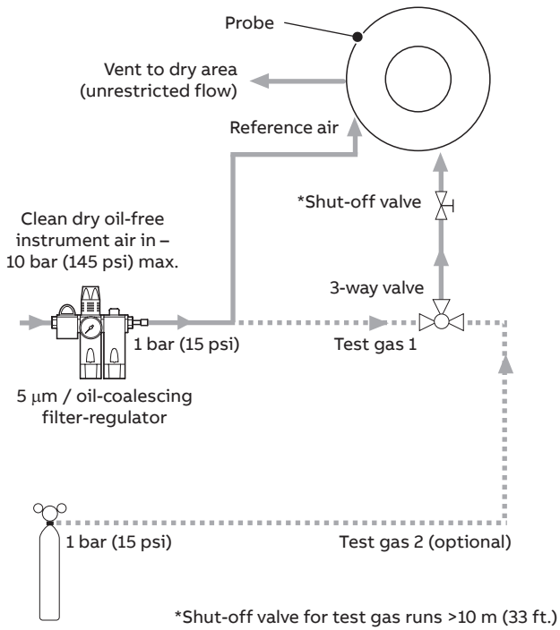
Non-AutoCal with air supply and restrictors
