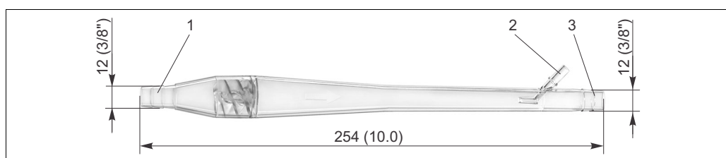
Fig. 37: Bubble trap, dimensions in mm (inch)
