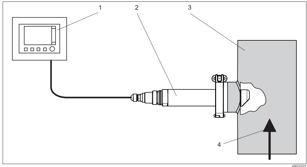
Fig. 6: Measuring system with flow assembly CUA262
