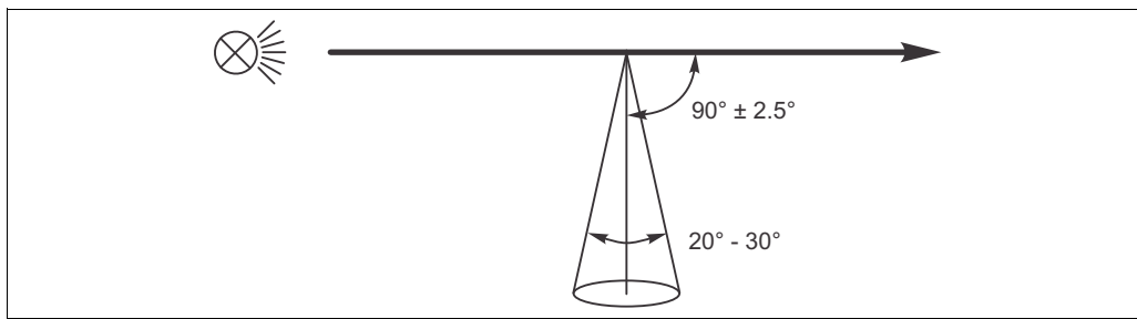
Fig. 25: Measurement in accordance with ISO 7027
