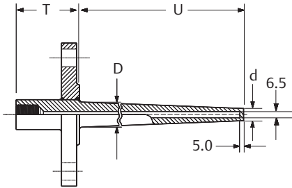
Figure 10. Flanged Barstock Thermowell – Tapered
